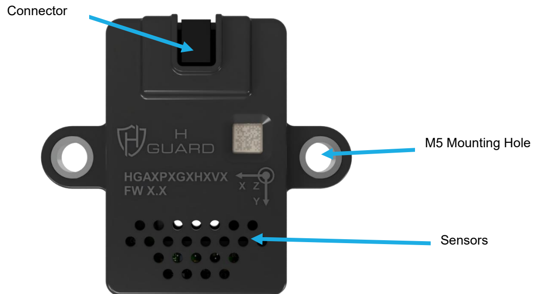
FIGURE 5 EXTERNAL FEATURES
