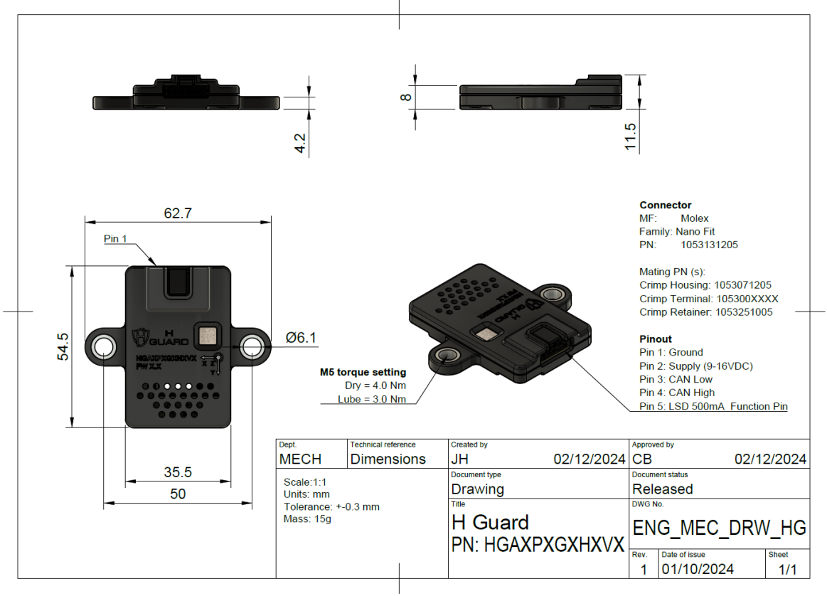
FIGURE 4 SENSOR DIMENSIONS
