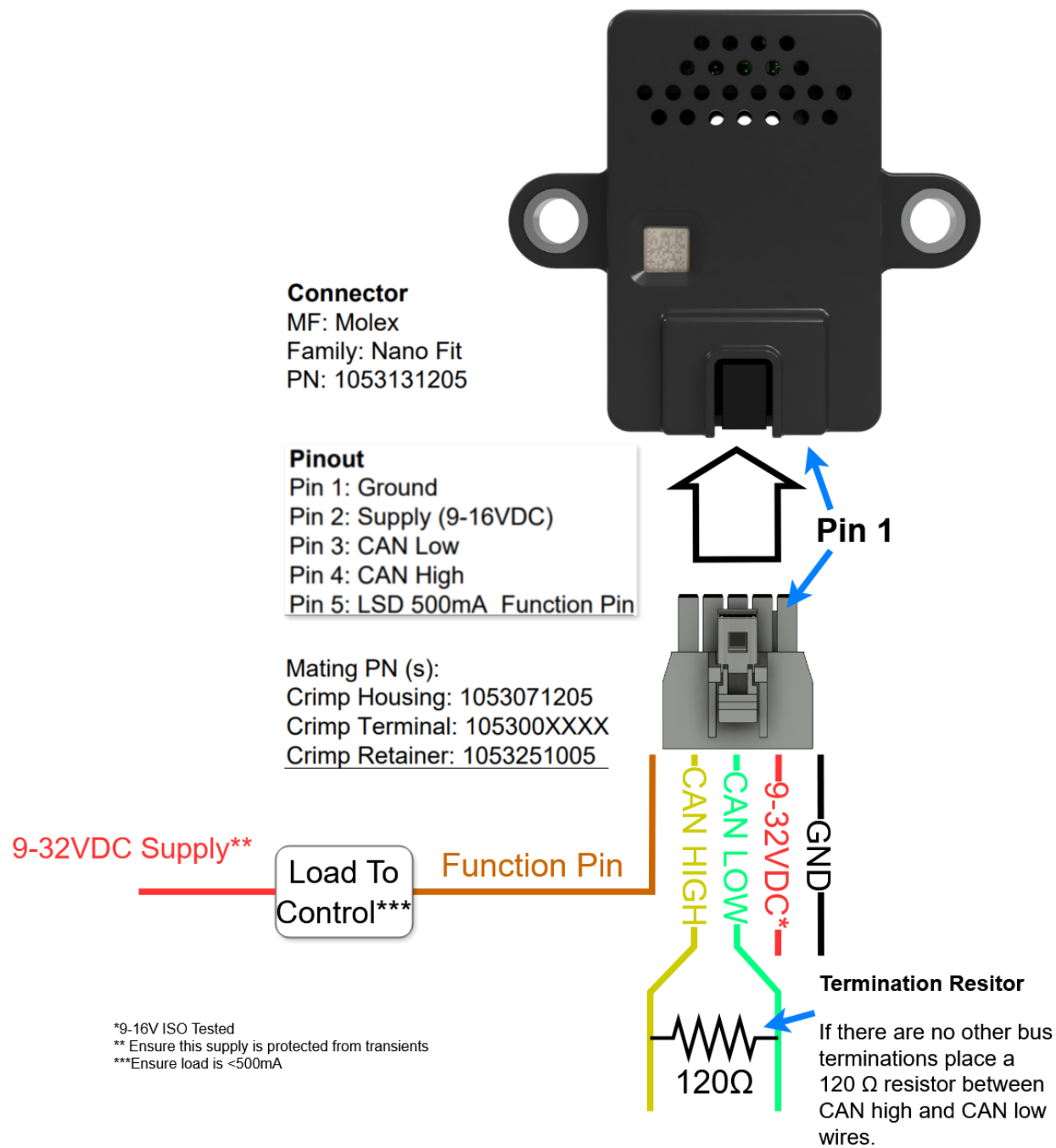
FIGURE 3 WIRING EXAMPLE
