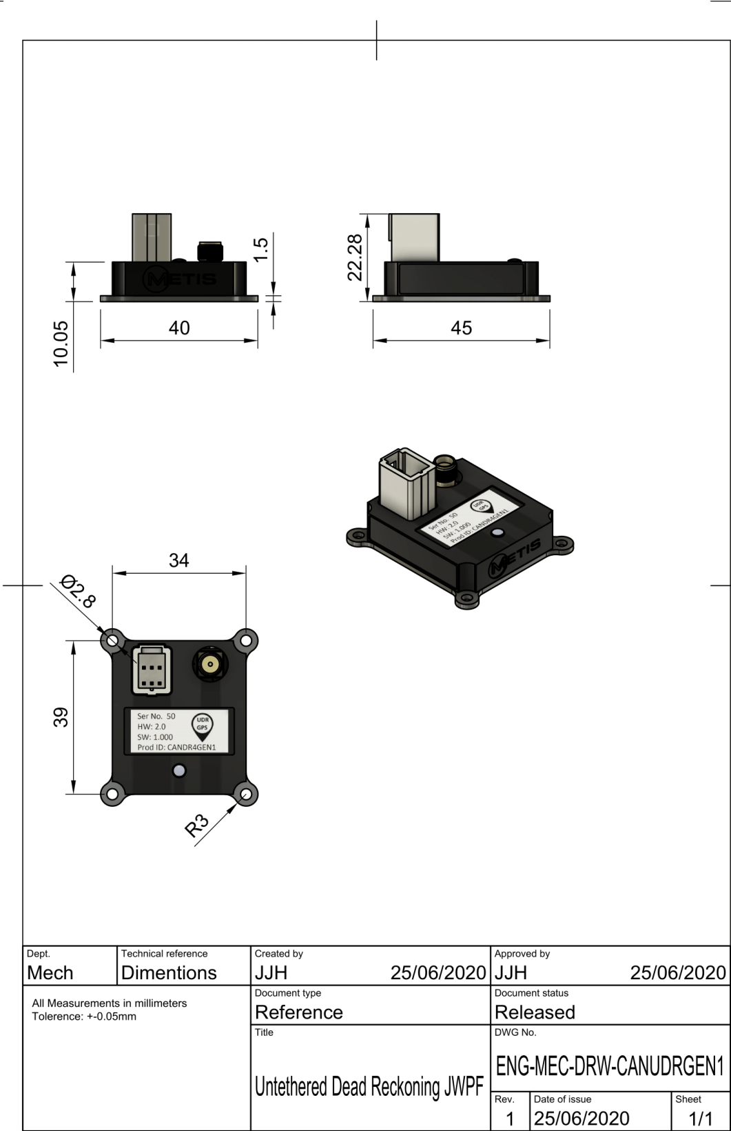
FIGURE 3 JWPF SENSOR DIMENSIONS
