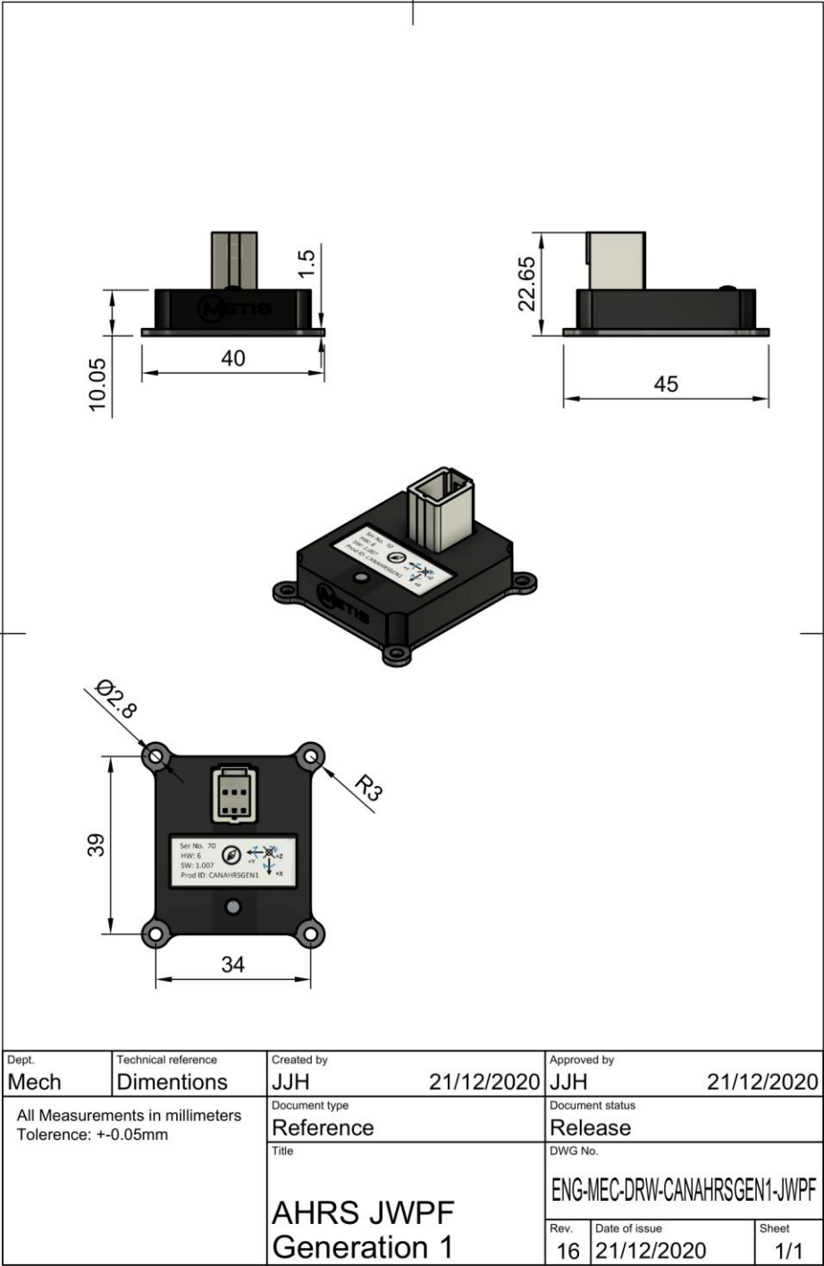
FIGURE 3 JWPF SENSOR DIMENSIONS
